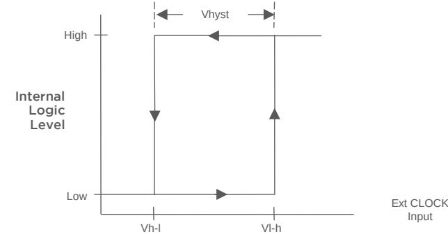
Figure 2: Hysteresis Diagram
