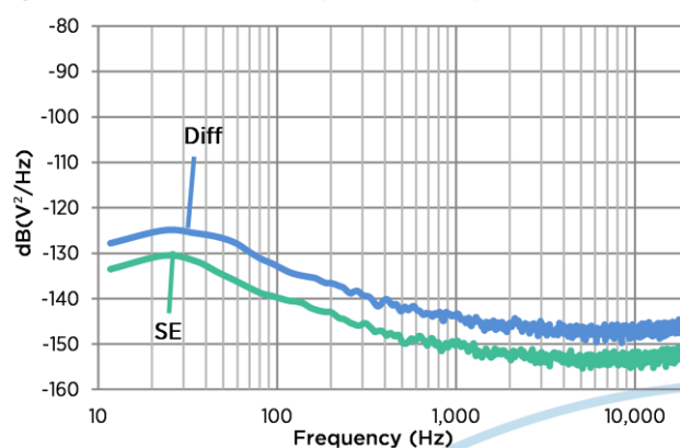
Figure 11: Noise Floor Power Spectral Density (NM)
