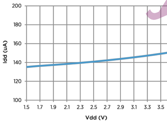
Figure 7: Typical Idd vs Vdd
