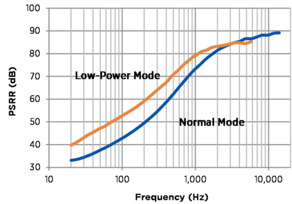
Figure 13: Typical PSRR
