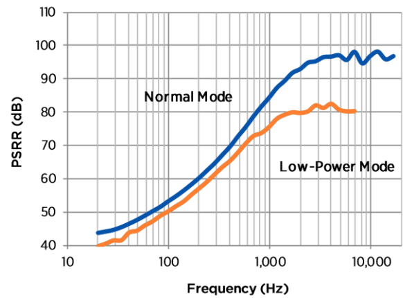
Figure 13: Typical PSRR
