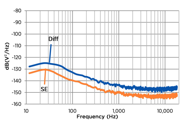
Figure 11: Noise Floor Power Spectral Density (NM)
