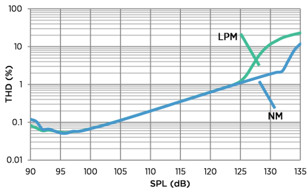
Figure 4: Typical THD vs Input SPL
