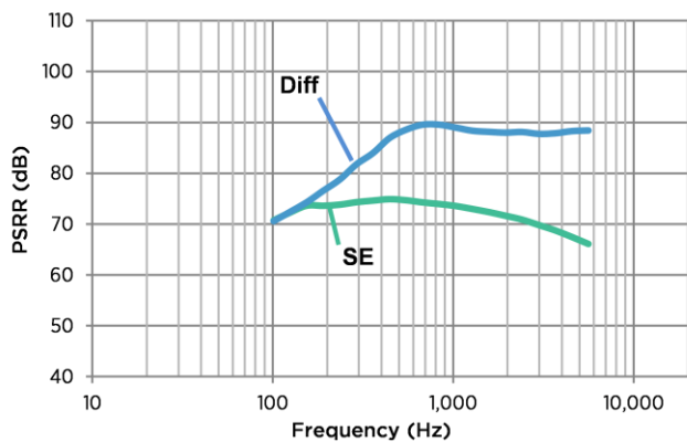
Figure 9: Typical PSRR (LPM)
