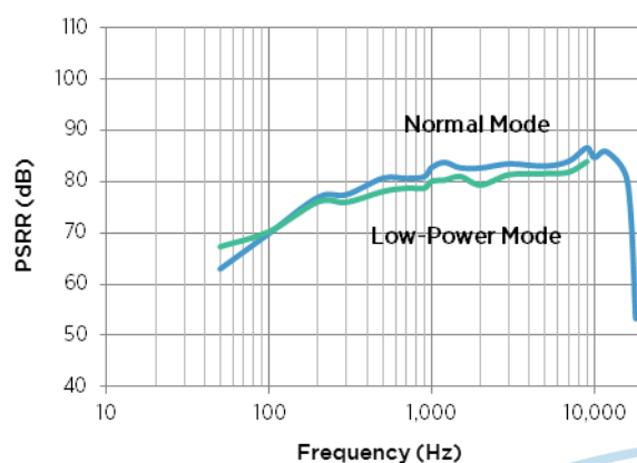
Figure 12: Typical PSRR
