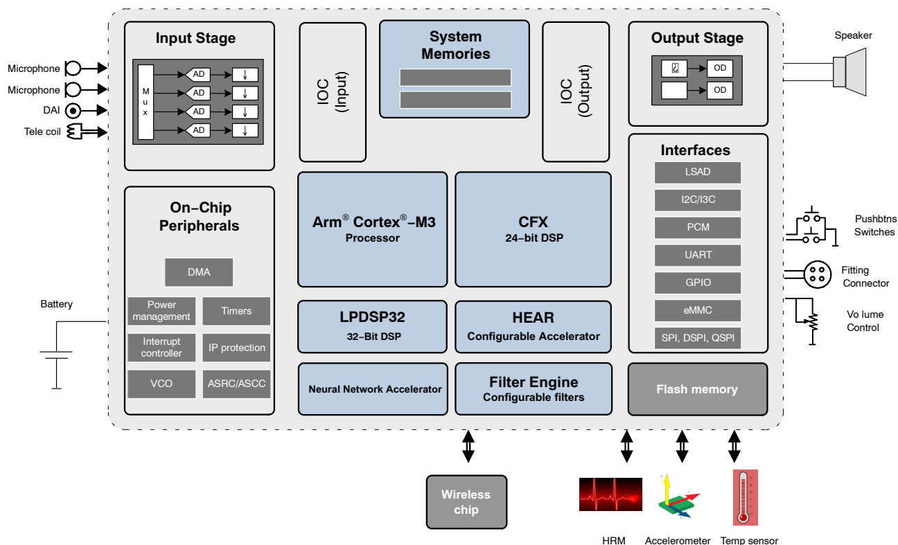
Figure 1. Ezairo 8310 Hybrid System Diagram
